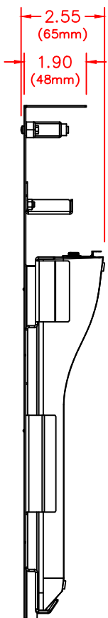
SIDE VIEW
