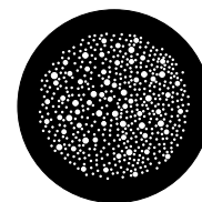
Code:190257000136 OD: Ø25.7 Pattern: Ø21 T=1.1mm Position: 7
