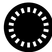
Code:190257000137 OD: Ø25.7 Pattern: Ø21 T=1.1mm Position: 6
