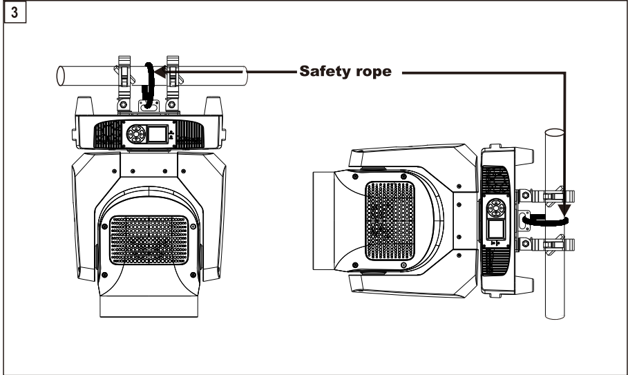
Installing the projector- Fig. 3
